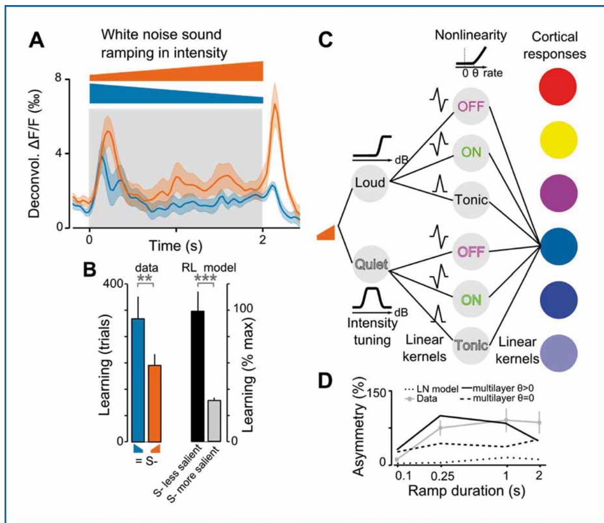
Figure 3: Asymmetric salience of up- and down-ramping sounds
