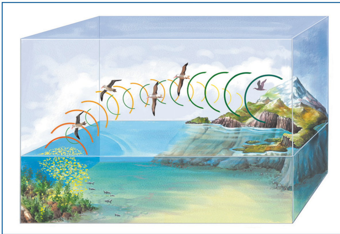
Figure 2. Olfactory landscape. Productive areas are often associated with bathymetric features, such as upwelling zones and sea mountains. Here, DMS emissions are higher and can provide olfactory signposts for navigation to a wandering seabird (From Thivent and Bonadonna, 2003 © Caroline Picard).
